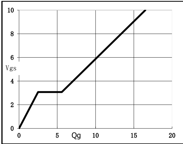
Fig.1 Gate-Charge Characteristics
